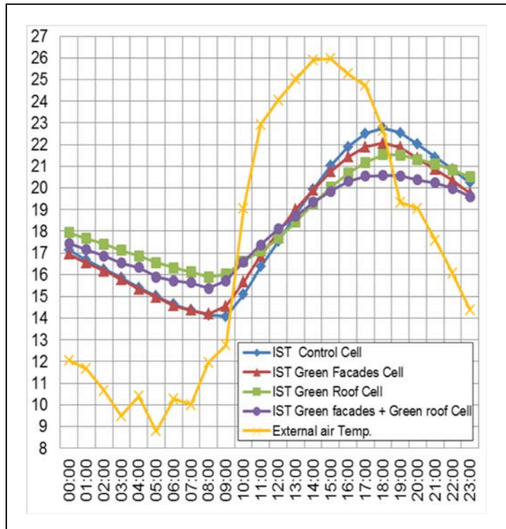
Figure 13. Internal surface temperature of west facades vs. external air temperature chart. Source: Own author Source: Own author.
