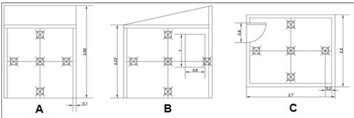
Figure 8. Distribution of thermocouple type T (Copper-Constantan). A-In West facades. B-In North facades. C-In roofs. Source: Own composition (Unscaled)
