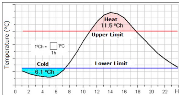
Figure 11. Degrees/hours of discomfort. Source: (Roriz et al., 2009)
