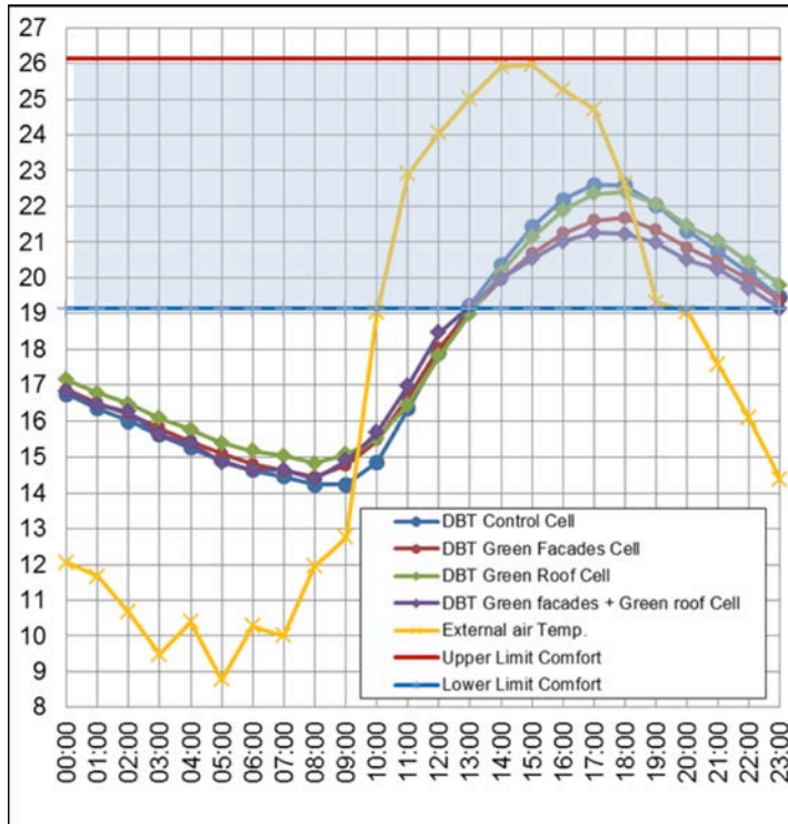
Figure 10. Evolution of internal air temperatures. Source: Own Composition
