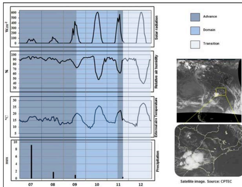
Figure 9. Climate Analysis. Episode 7-12 July 2015. Source: Own author
