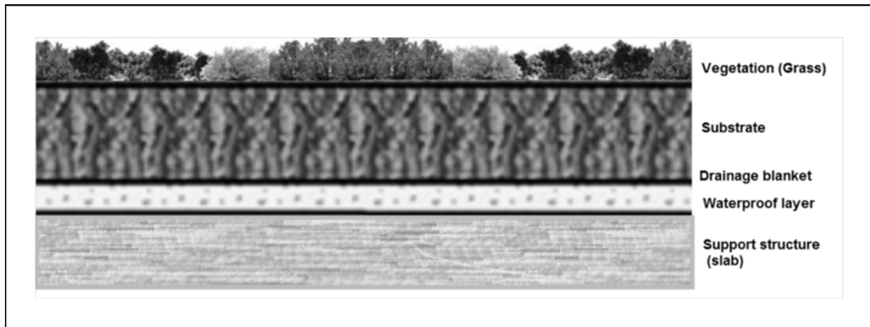
Figure 5. Profile of Green roof. Source: Own composition
