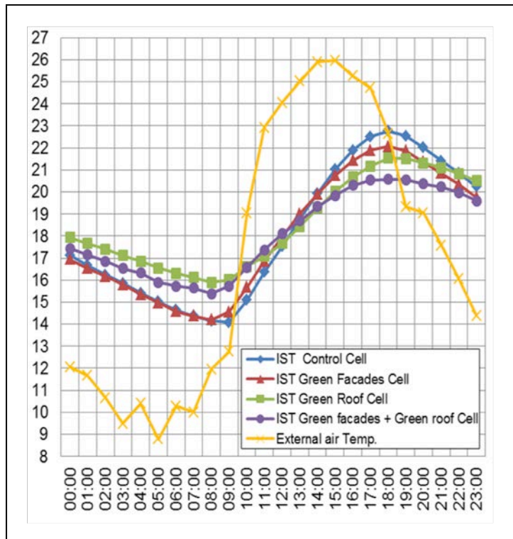
Figure 14. Internal surface temperature in roofs vs. external air temperature. Source: Own author
