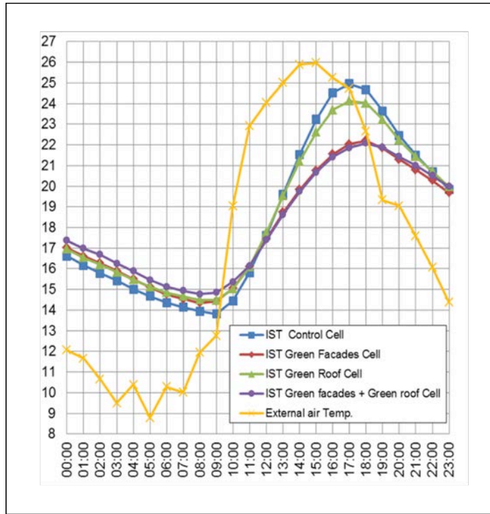
Figure 12. Internal surface temperature's north facades vs. external air temperature: Graphic. Source: Own author
